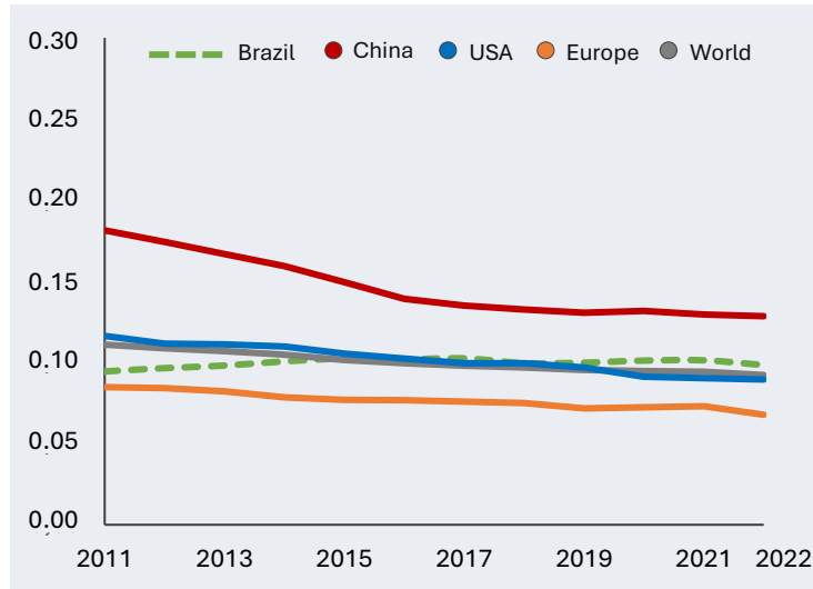
Energy intensity of TES [toe/thousand US$ppp (2021)]
