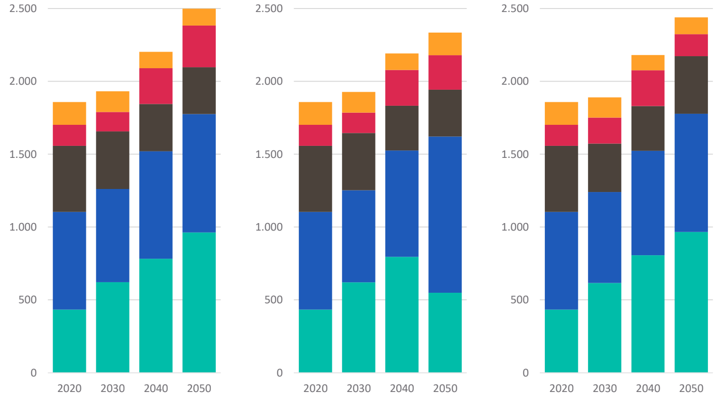
Total energy use by industry (PJ)
